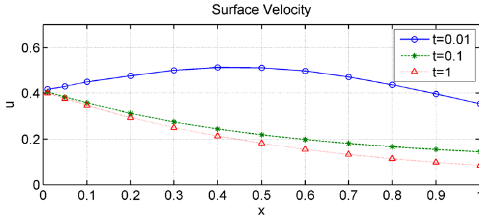
Figure 44 Velocity at the free surface at instances t=0.01 , t=0.1 and t=1 ( \Delta T=22^\circ\text{C} , \tau=3.5\text{s} , A=0.03 , U=15\text{mm/s} , Bo=2.8 \times 10^4 , Ma=2.5 \times 10^4 , Re=290 )
