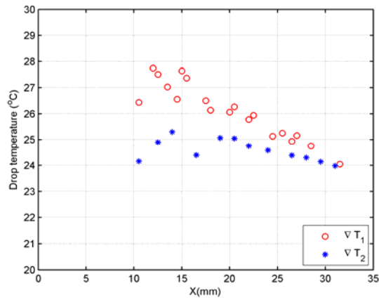
Figure 34 Effect of thermal gradient and size (volume) on motion of lens drops; q_{in,1}=11.9W , q_{in,2}=4.3W . Internal temperature of the drop is found by spatio-temporal interpolation of thermocouple readings. Left column graphs are for drop size: 2\mu L and right column graphs are for drop size: 10\mu m .
